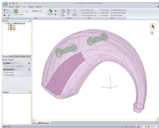
Figure 1 CAD drawing of the Inteco IN-m hearing aid including details of the microphone inlets.
